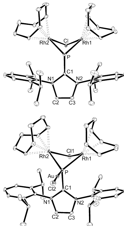
Figure 5. ORTEP diagram of 9 (top) and 9-AuCl (bottom) with thermal displacement parameters drawn at 50% probability level. Selected bond length [Å] and angles [°]: In 9 : Rh1–P 2.3613(4), Rh1–Cl 2.4349(4), Rh2–P 2.3689(4), Rh2–Cl 2.4302(4), P–Cl 1.8056(17); P–Rh1–Cl 84.426(14), P–Rh2–Cl 84.368(14), Rh1–P–Rh2 75.391(12), Rh1–Cl–Rh2 72.957(11), C1–P–Rh1 110.43(5), C1–P–Rh2 107.79(5), N1–C1–N2 104.02(14). In 9-AuCl : Rh1–P1 2.3457(13), Rh1–Cl1 2.4056(13), Rh2–P 2.3382(13), Rh2–Cl1 2.4268(13), P–Cl 1.855(5), Au–P 2.2712(12), Au–Cl2 2.3340(12); P–Rh1–Cl1 83.12(4), P–Rh2–Cl1 82.82(4), Rh1–P–Rh2 78.31(4), Rh1–Cl1–Rh2 75.47(4), C1–P–Rh1 112.46(15), C1–P–Rh2 115.48(15), N1–C1–N2 105.7(4), P–Au–Cl2 176.95(5).
