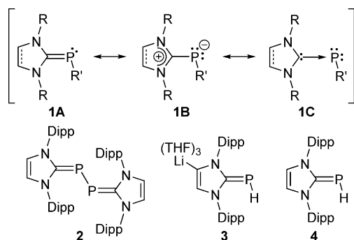
Figure 1. Selected N -heterocyclic carbene–phosphinidene adducts (2-phosphinideneimidazolines, Dipp = 2,6-diisopropylphenyl).
