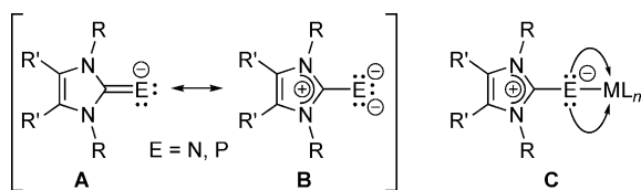
Figure 2. Resonance structures (A, B) of imidazolin-2-ynide ligands and their potential interaction with metals as 2σ,4π electron donors (C).
